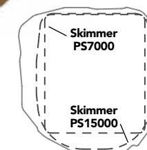
RL70 Footprint
